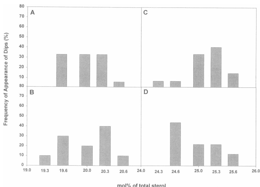
FIGURE 3 Distribution of DHE intensity dips observed in the neighborhood of 20 (A and B) and 25 (C and D) mol% total sterol in DHE/cholesterol/DMPC (A and C) and DHE/ergosterol/DMPC (B and D) mixtures. The frequency of appearance of dips was determined from 13 independently prepared samples for B and D and from 16 samples for A and C. The height of the column represents the frequency of appearance of the dip at the sterol concentration indicated underneath. The sample incubation time was 28 days. The average dip positions and their standard deviations were (A) 20.0 \pm 0.32 mol%, (B) 20.0 \pm 0.39 mol%, (C) 25.1 \pm 0.33 mol%, and (D) 25.0 \pm 0.37 mol% total sterol.
