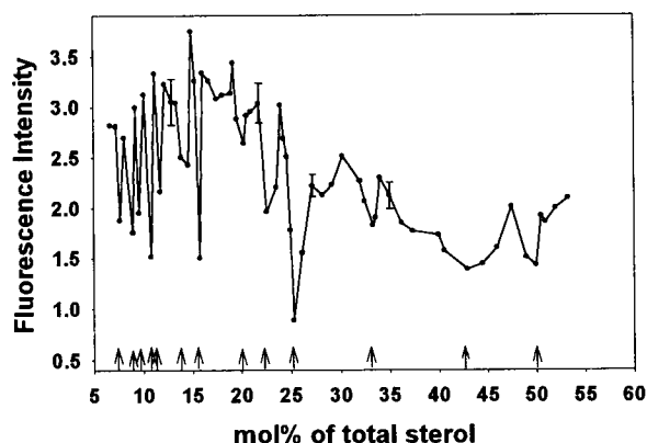
FIGURE 4 Effect of total sterol content on the DHE fluorescence intensity (measured at 35°C) at 378 nm in DHE/cholesterol/DMPC mixtures with DHE fixed at 0.5 mol%. The sample incubation time was 28 days.
